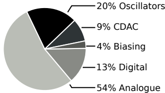
b) System Power: 1.28 \mu\text{W}
